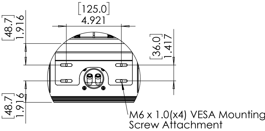
DETAIL G SCALE 1 : 5 VESA Mount M6 Attachment
