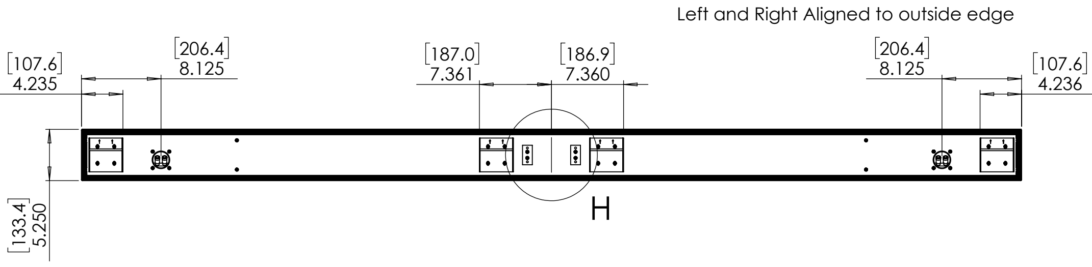
VESA Mount M6 Attachment DETAIL H SCALE 1 : 5
