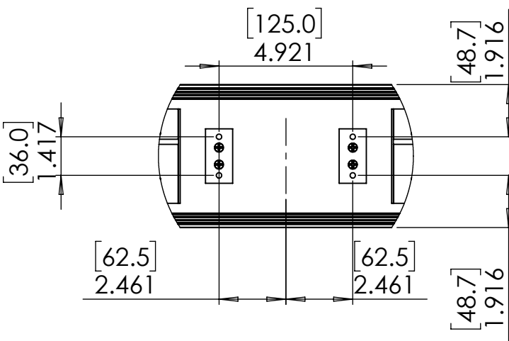
VESA Mount M6 Attachment DETAIL H SCALE 1 : 5
