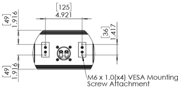
DETAIL G SCALE 1 : 5 VESA Mount M6 Attachment
