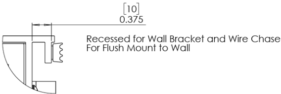
DETAIL F SCALE 1 : 1
