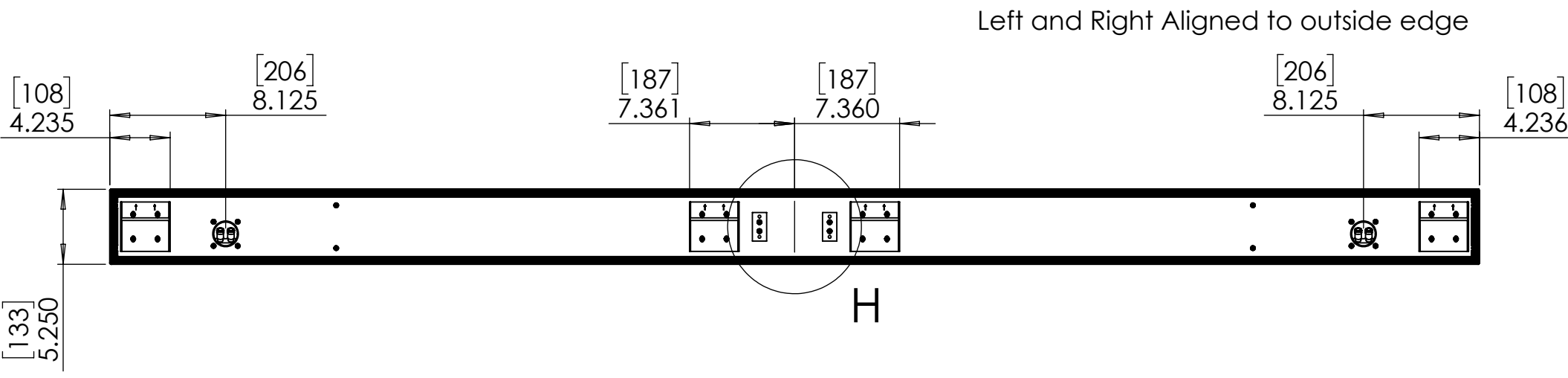
VESA Mount M6 Attachment DETAIL H SCALE 1 : 5
