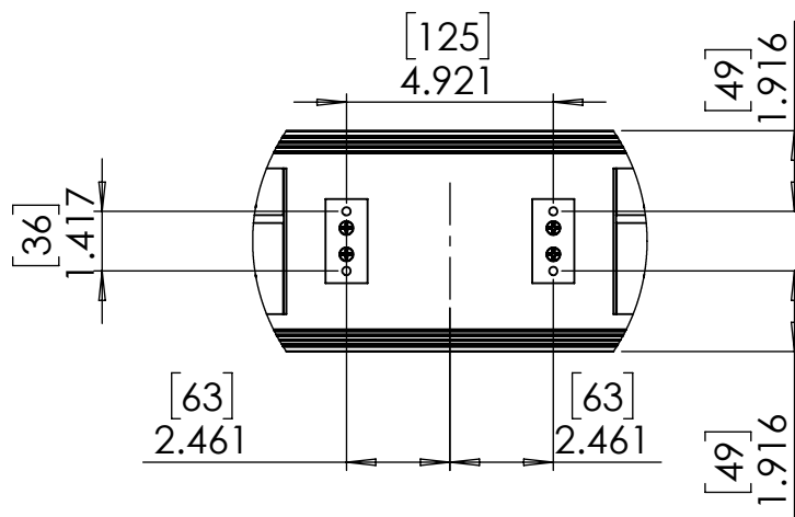
VESA Mount M6 Attachment DETAIL H SCALE 1 : 5
