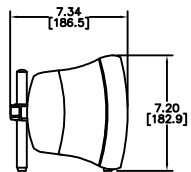
SIDE
