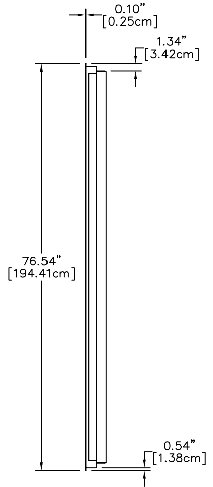
GRILL ON DIMENSIONS SIDE VIEW
