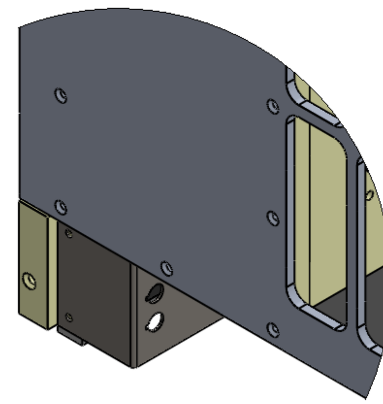
Removable Assess Panel for Terminal Connection DETAIL A SCALE 1 : 2
